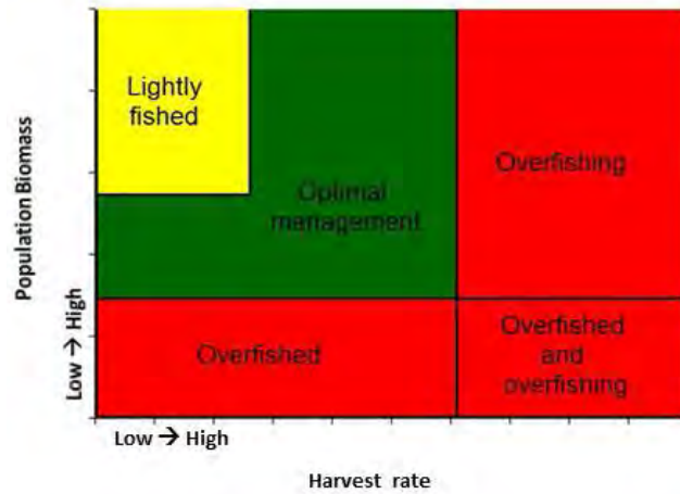
Figure 4-2: The general relationship between harvest rate and stock size.
