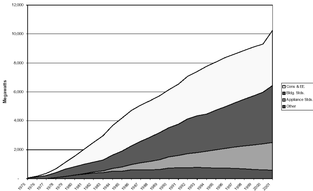
Figure A-10 Peak Demand Impacts of Energy-Efficiency Programs and Standards
