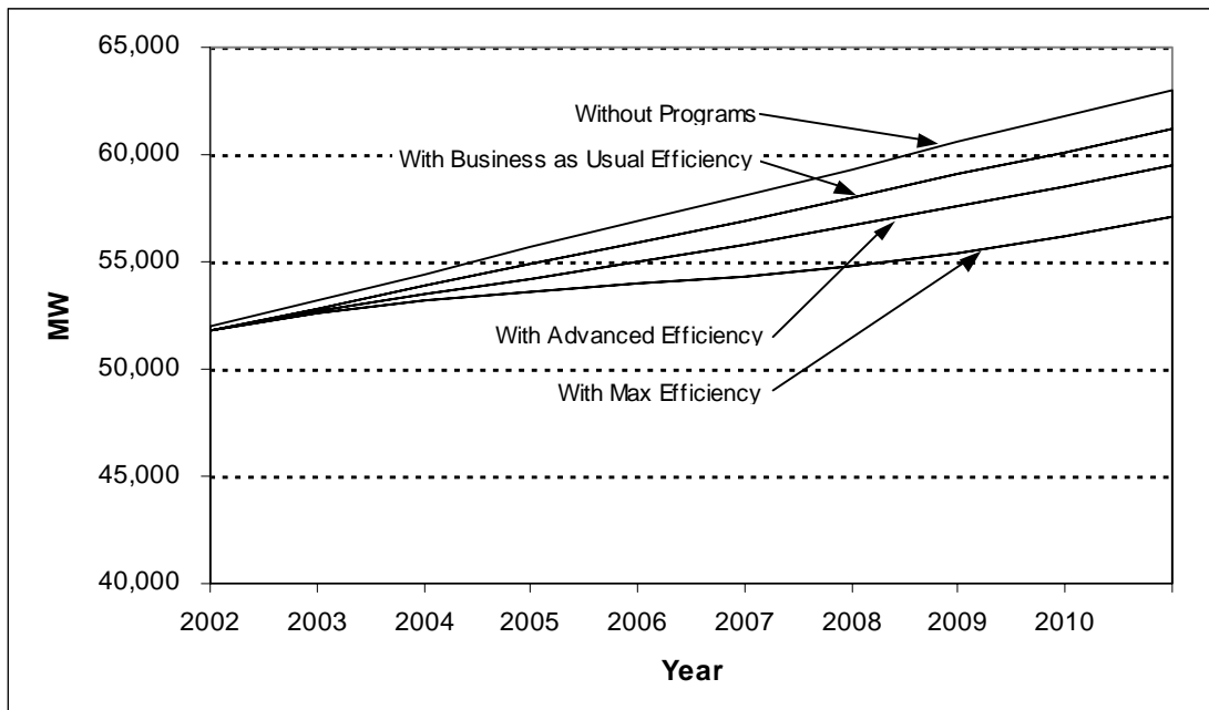
Figure 3-6 Peak Demand Forecast and Achievable Efficiency Potentials*
