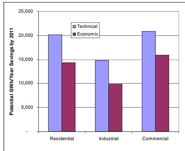
Figure 3-11 Technical and Economic Potential (2011) Energy Savings by Sector—GWh per Year
