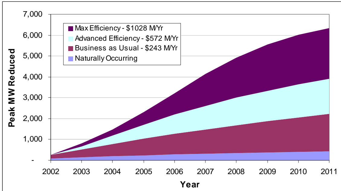
Figure 3-5 Achievable Peak Demand Savings—MW
