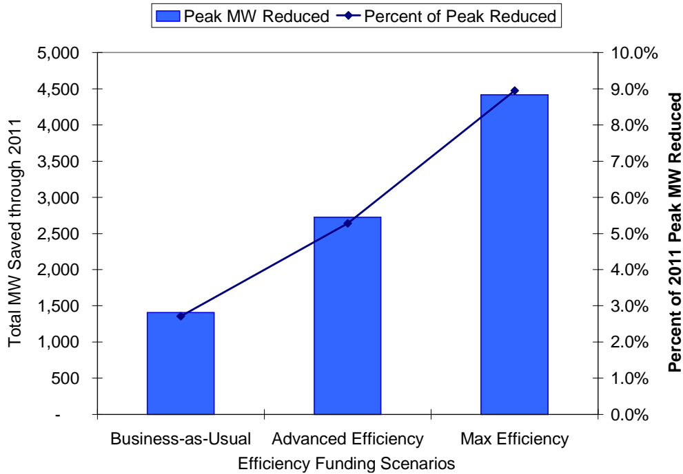
Figure ES-2 California Peak Demand Forecast and Efficiency Potentials
