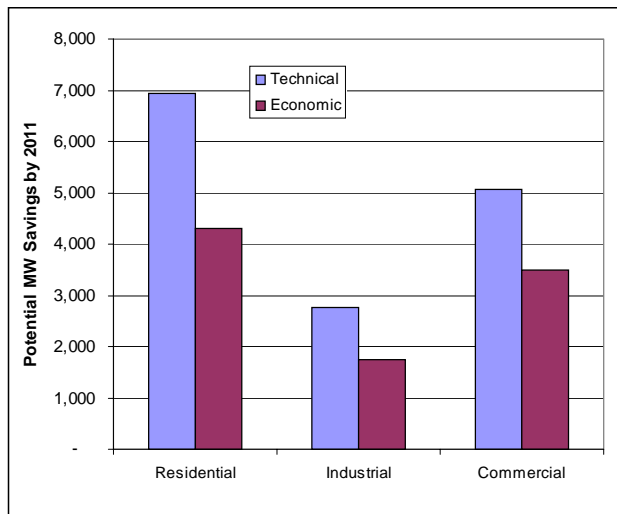
Figure 3-10 Technical and Economic Potential (2011) Demand Savings by Sector—MW
